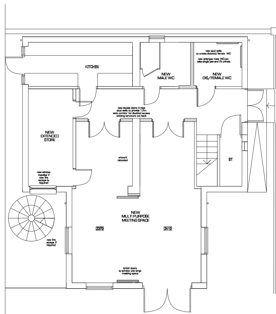
GROUND FLOOR PLAN AS PROPOSED
