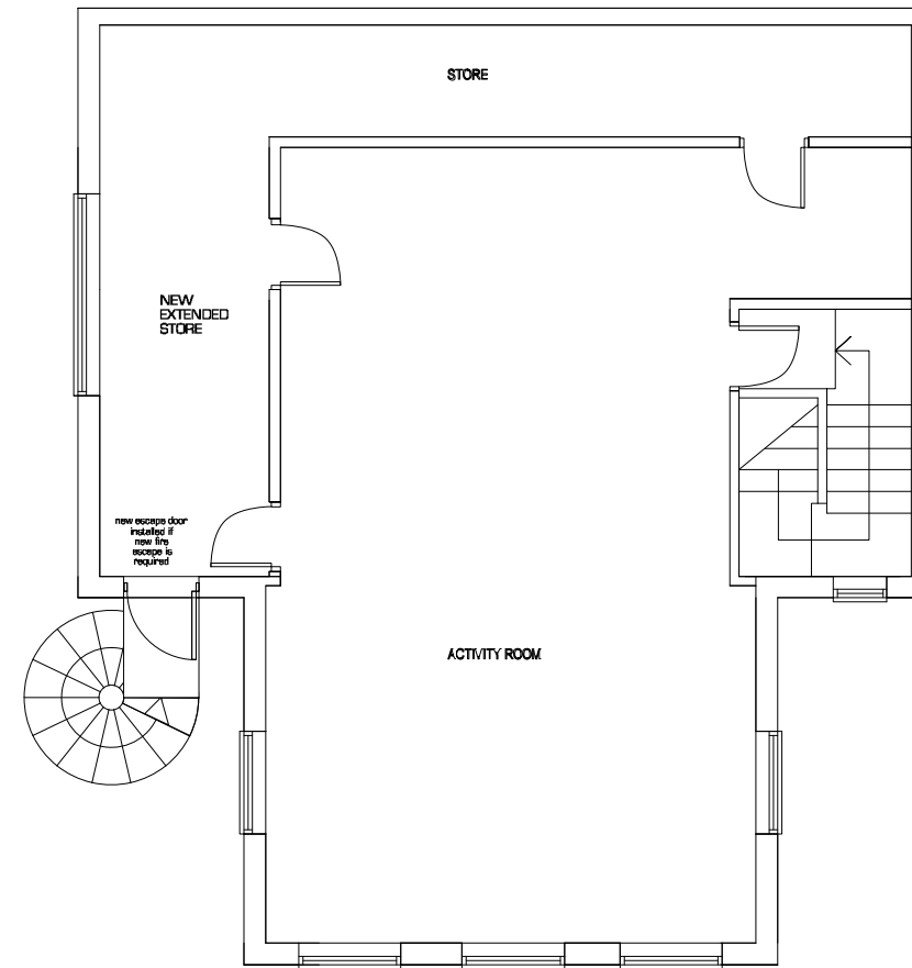
FIRST FLOOR PLAN AS PROPOSED
