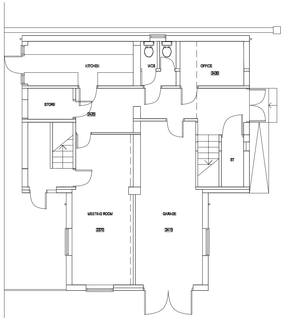
GROUND FLOOR PLAN AS EXISTS
