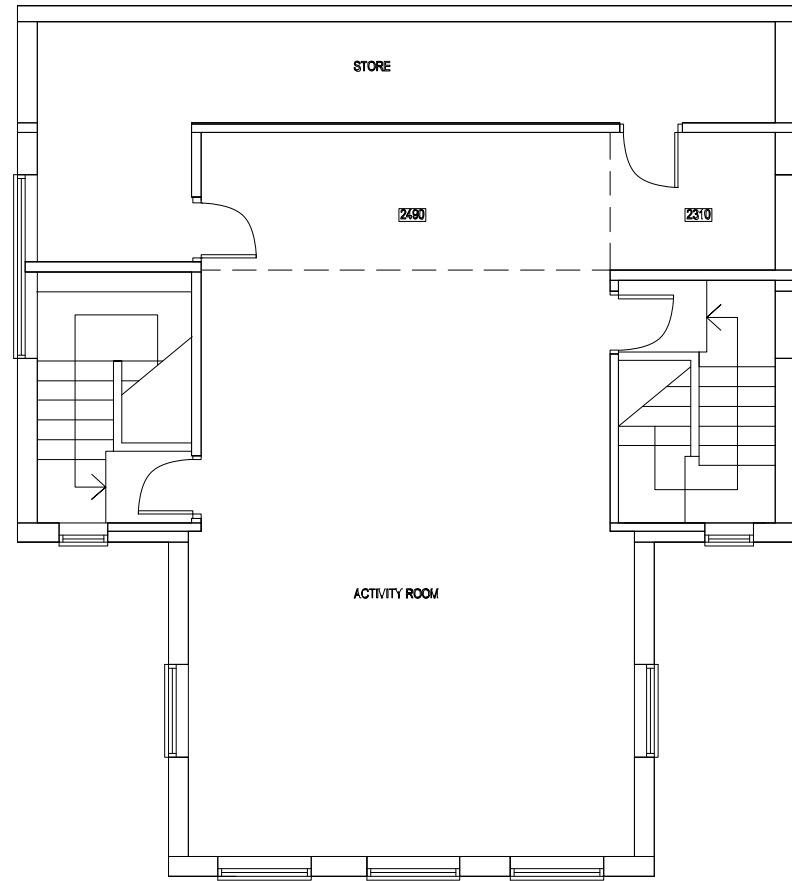
FIRST FLOOR PLAN AS EXISTS
